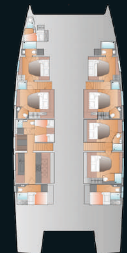
6 GUESTS + CREW QUARTERS
