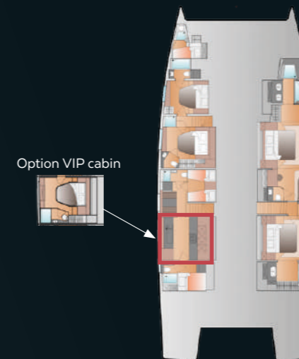
MAESTRO + VIP + 2 GUESTS + CREW QUARTERS
